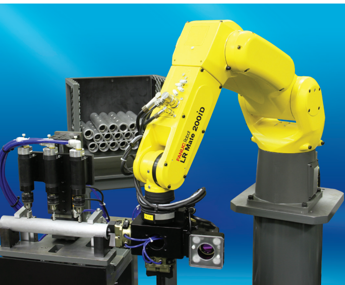
Intelligent deburring
